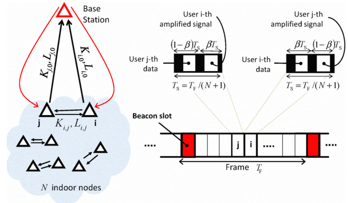
Figure 1. Propagation setting (left). TDMA framing structure (right).
