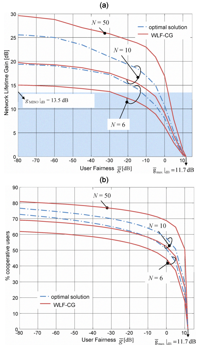
Figure 2. (a) Average network lifetime (energy) gain vs. the user-fairness constraint. Outside the shaded region the proposed system performs better than Alamouti transmission in a 2 \times 1 MISO system. (b) Average percentage of cooperative users vs. the user-fairness constraint.
