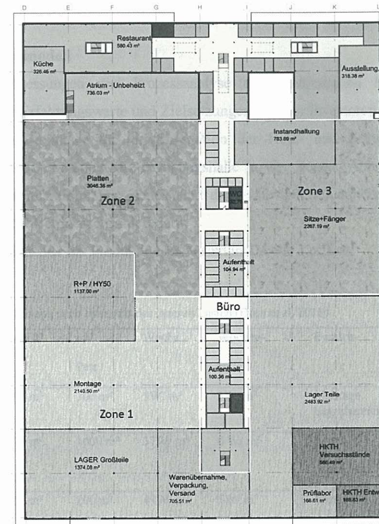
Abb.5: Grundriss EG
