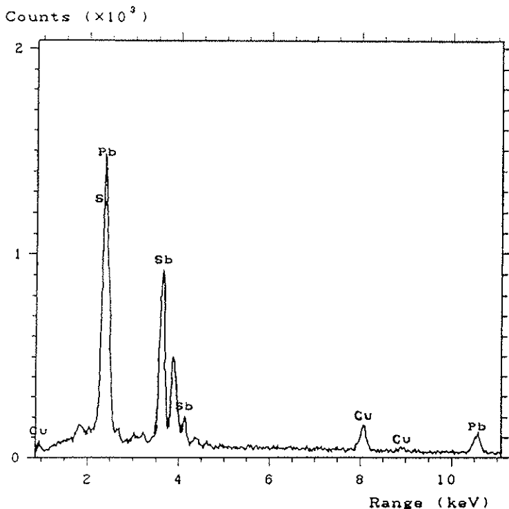
Fig. 9. Surface analysis.
