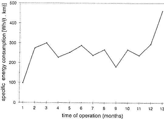
Fig. 3. Mean values of specific energy consumption vs. time of operation.
