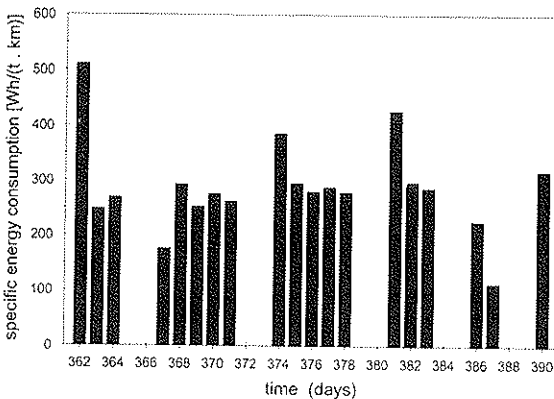
Fig. 4. Specific energy consumption at intermittent operation.
