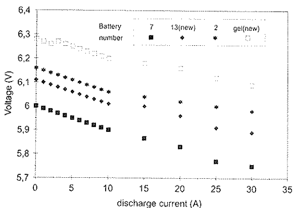
Fig. 6. Current-voltage characteristics.
