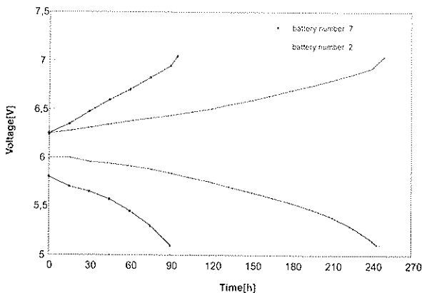
Fig. 5. Charge/discharge cycles.
