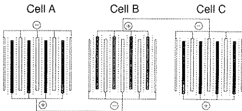
Fig. 2. Schematic cell design.
