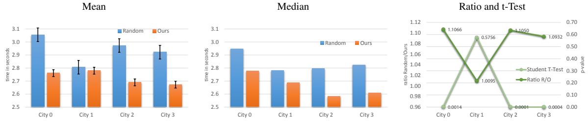
Figure 4: The results of the response of over 50 users in the layout readability test described in Section 7.1. The black bars in the first chart indicate the standard error. The last chart shows the ratio R/O and the p-value of the Student’s t-test.
