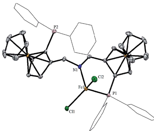
Fig. 3 Structural view of ( S_{\text{FC}},S_{\text{FC}} )-13c showing 50% thermal ellipsoids (H atoms and solvent molecules are omitted for clarity). Selected bond lengths (Å) and bond angles (°): Fe1–Cl1 2.2438(8), Fe1–Cl2 2.2472(8), Fe1–P1 2.4031(8), Fe1–N1 2.095(2), Cl1–Fe1–Cl2 119.83(3), P1–Fe1–Cl1 110.96(3), P1–Fe1–Cl2 112.63(3), Cl1–Fe1–N1 113.32(7), Cl2–Fe1–N1 106.64(7).
