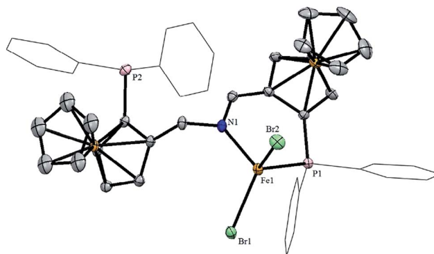
Fig. 2 Structural view of ( S_{\text{FC}},S_{\text{FC}} )-13a showing 50% thermal ellipsoids (H atoms and solvent molecules are omitted for clarity). Selected bond lengths (Å) and bond angles (°): Fe1–Br1 2.3818(5), Fe1–Br2 2.3916(5), Fe1–P1 2.3999(9), Fe1–N1 2.090(3), P1–Fe1–Br1 110.42(3), P1–Fe1–N1 95.16(8), Br1–Fe1–N1 115.47(8), Br2–Fe1–P1 112.84(3), Br2–Fe1–N1 102.08(8).
