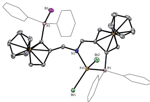
Fig. 7 Structural view of (S_{Fc}, S_{Fc}) -14 showing 50% thermal ellipsoids (H atoms and solvent molecules are omitted for clarity). Selected bond lengths ( \text{\AA} ) and bond angles ( ^\circ ): Fe1–Br1 2.3911(7), Fe1–Br2 2.3887(6), Fe1–P1 2.400(1), Fe1–N1 2.088(3), P2–B1 1.927(5), Br1–Fe1–Br2 117.74(3), P1–Fe1–Br1 110.70(3), P1–Fe1–Br2 112.80(3), Br1–Fe1–N1 115.53(9), Br2–Fe1–N1 102.68(9).
