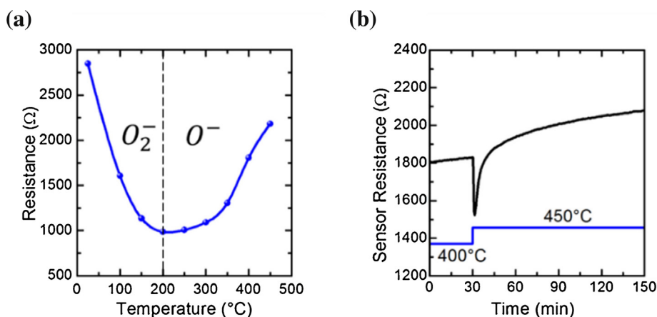
Fig. 3. (a) Resistance of SnO 2 locally grown NWs as a function of temperature. The minimum in resistance reflects the change in the adsorbed oxygen specie; (b) Transient response of the sensor resistance in a change of temperature illustrating the increase in resistance for increasing temperatures above 200 °C. Blue line represents the evolution of temperature.
