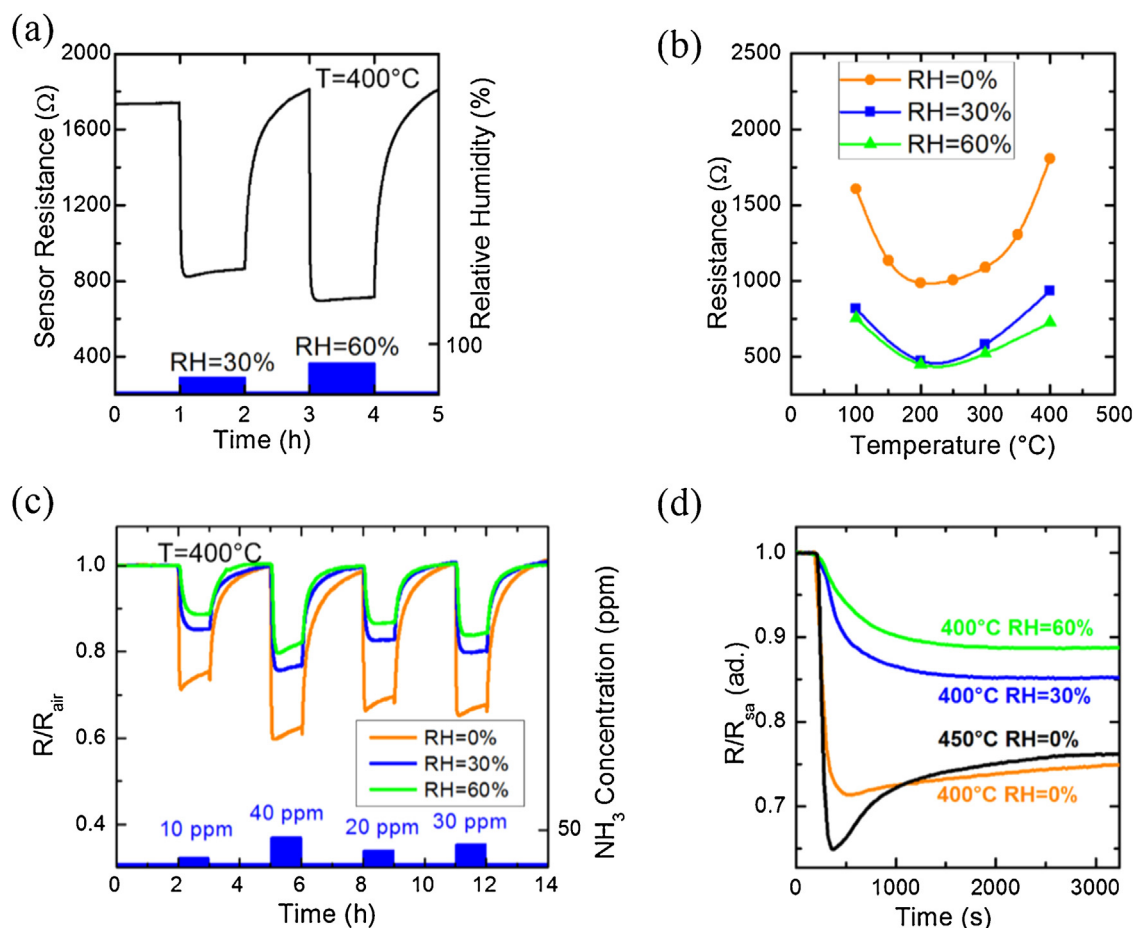
Fig. 5. (a) Electrical response of SnO 2 NWs to different concentrations of water vapor in synthetic air at 400 °C; (b) Resistance of SnO 2 NWs for different humidity levels at different temperature. U-shaped R-T is also obtained in humid conditions due to dissociation of molecular to atomic oxygen at a temperature of 200 °C; (c) Electrical response of SnO 2 NWs in dry, 30% and 60% of relative humidity (RH at room temperature) towards different ammonia pulses in synthetic air. Three tests have been performed by keeping 400 °C constant temperature; (d) Sensor response towards 10 ppm of NH 3 at different conditions. The overshoot in resistance is visible for 450 °C and RH=0% curve.
