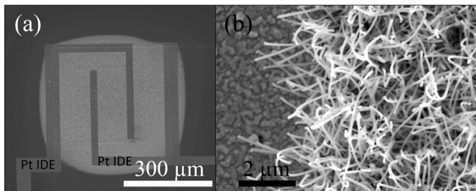
Fig. 1. (a) SEM general view of the micromembrane with Pt interdigitated electrodes (IDE) on the top. Brighter area corresponds to the grown SnO 2 NWs; (b) SEM image of SnO 2 NWs contacting the Pt electrode (on the left side);.
