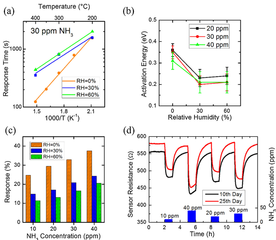
Fig. 6. (a) Response time of sensor of NH 3 pulses of 30 ppm in dry and humid condition, represented in an Arrhenius plot. Symbols are experimental values and lines are the fitted exponential decay; (b) Activation energy obtained from response time for ammonia response in function of relative humidity, for all the concentrations studied; (c) Response in humid condition of SnO 2 NWs against ammonia at 400 °C. The sensor distinguishes the concentration of ammonia in a precision of 30 ppm in realistic operational conditions, where humidity is present; (d) Comparison between the response of the sensor at 300 °C and 30% of RH from 10th and 25th day of measurements. A change of 5% in resistance baseline is obtained.
