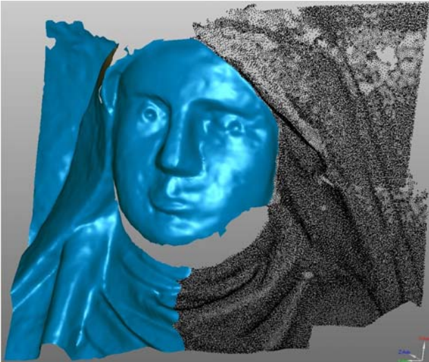
Figure 4: Surface model with 1mm resolution, covering about 30×25cm 2 , derived from the Minolta data using ca. 125 thousand points. The left part is triangulated, the right one shows the points used.
