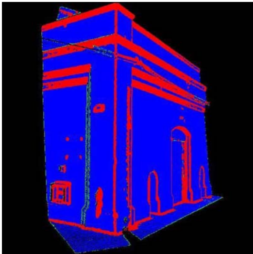
Figure 1: Classified point cloud; Blue: points representing surfaces; Red: Points representing edges; Green: Points representing boundaries. (Belton and Lichti, 2006).
