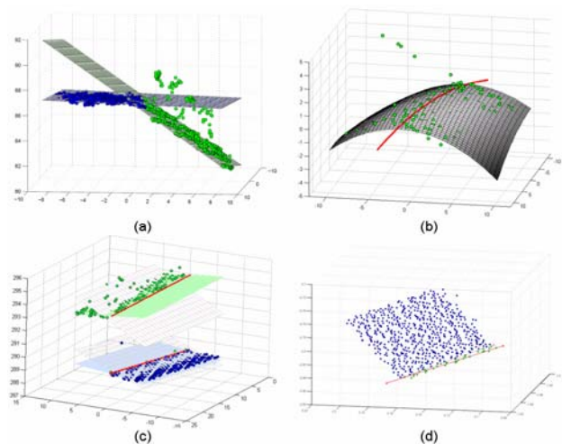
Figure 4: Practical examples for the modelling of different feature line types; break line with 2 intersecting robust planes (a), form line determination based on a robust quadric adjustment (b), step edge modelling with 2 non-intersecting planes (c), and boundary line based on just one plane and missing data on the other side of the line (d). (Briese and Pfeifer, 2008)
