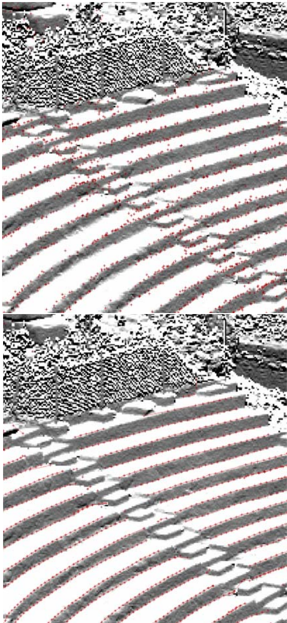
Figure 5: Shading of the 2.5D surface model derived from the polar observations overlaid with vector data; Upper image: automatically extracted start-segments (every twentieth TLS point was analysed); Lower image: automatically extracted feature lines with the proposed approach.
