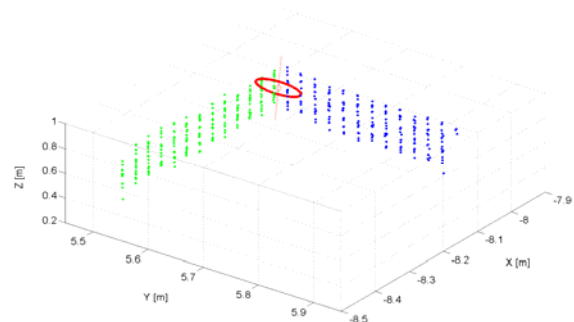
Figure 6: Covariance ellipsoid for one break line patch; Red: resulting break line (dotted line), representative point on the break line (diamond) and corresponding error ellipsoid (principle axis: 0.014m and 0.007m enlarged by a factor of 3); Green: TLS points of the left patch; Blue TLS points of the right patch. (Briese and Pfeifer, 2008)
