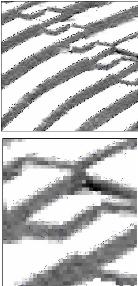
Figure 3: Result of the feature line detection of a staircase. The background image shows the polar TLS data domain from one stand point with a “pixel size” of 0.03° at a distance of about 65m from the sensor. It is displayed as a shading of the 2.5D surface model determined from the polar observations. The feature line detection is based on quadric analysis. Next to the detected 3D location of the feature line (symmetry point) the feature line direction (represented by the second point) was estimated; Upper part: overview; Lower part: detail.
