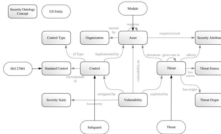
Fig. 3. Relationships among Grundschrift entities and security ontology concepts
