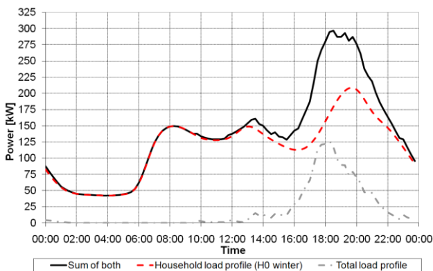
Figure 4: The total load profile for uncontrolled charging of 100 BEV, the load profile of 200 households and the sum of both. Charging after the last trip in the considered grid (settlement)
