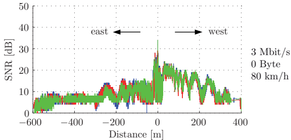
Fig. 3. SNR plot for vehicle driving west, transmit power 15.5 dBm
