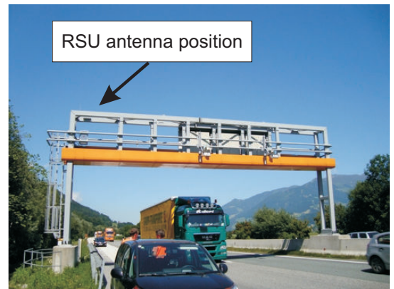
Fig. 1. Measurement scenario including RSU antenna position
