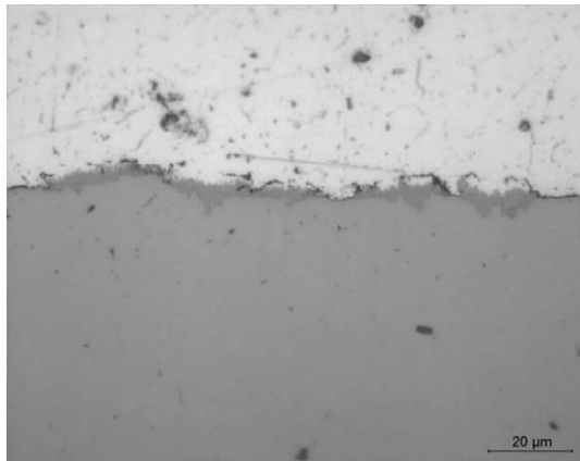
Figure 7. (a) Micrograph of the aluminum-steel interface of a bimetal-wire produced by laser assisted roll bonding. IMPs and several small cracks are visible. (b) Results of tensile tests of bi-metal-wire laser welded samples. Bi-metal-wire laser welded samples have been compared to steel-steel and aluminum-aluminum laser welds. The tensile strength of bi-metal-wire samples increased slightly in comparison to Al99.0.
