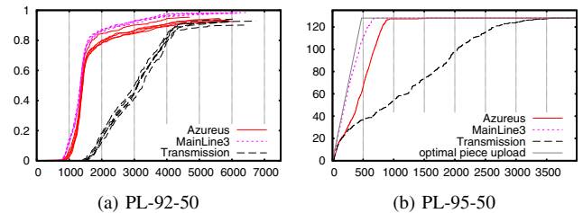
Fig. 2. (a) Experiment repeated 5 times with identical settings. [x = time in seconds; y = fraction of clients] (b) Unique pieces uploaded by initial seed. [x = time in seconds; y = MiB]
