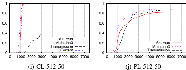
Fig. 1. Download time CDFs for different experiments. (cont.)
