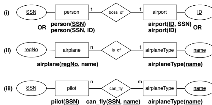
Fig. 6. The cardinalities of relationships of ER diagrams.
