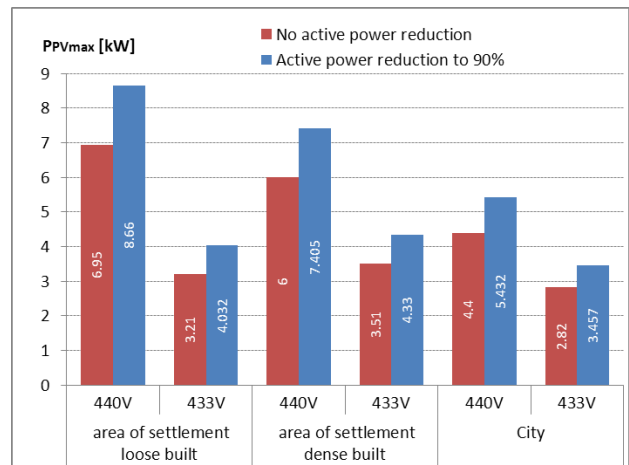
Figure 13: Active power reduction
