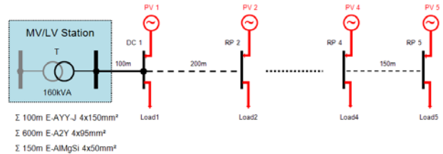
Figure 9: LV-Network – Area of settlement loose built
