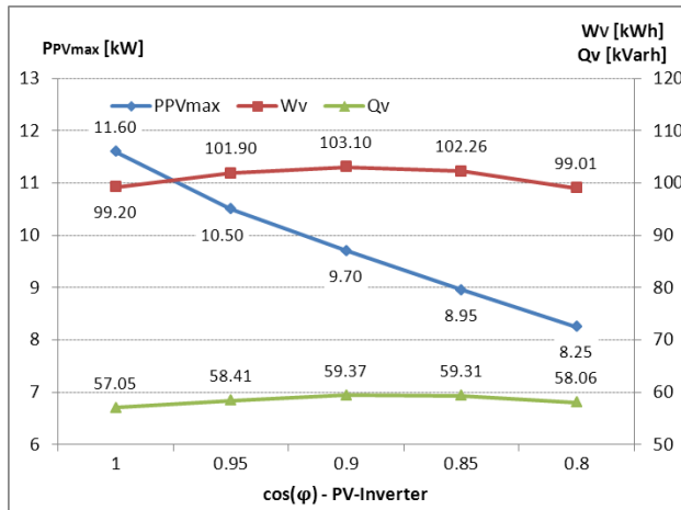
Figure 4: City – Tap -10%
