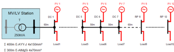
Figure 5: LV-Network – Area of settlement dense built
