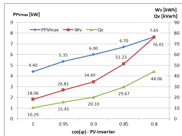
Figure 2: City – Tap 0%
