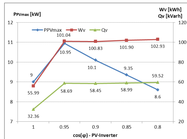
Figure 3: City – Tap -5%
