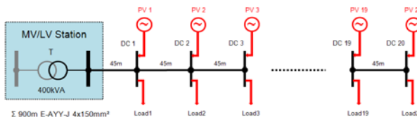
Figure 1: LV-Network - City
