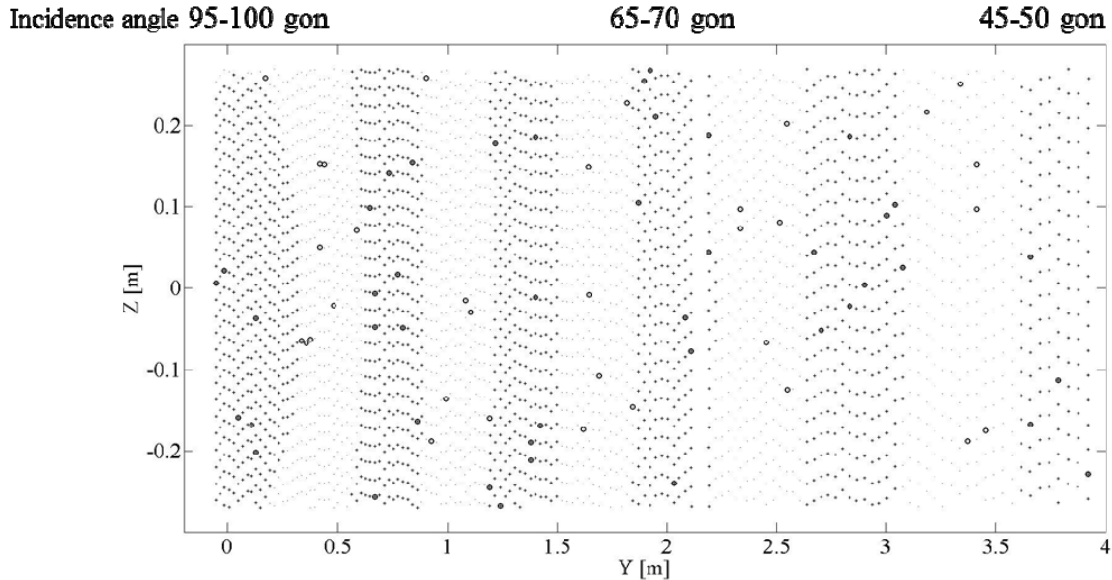
Fig. 2: Point cloud of the measured object, segmented zones and points selected to be determined with TMS (circles)
