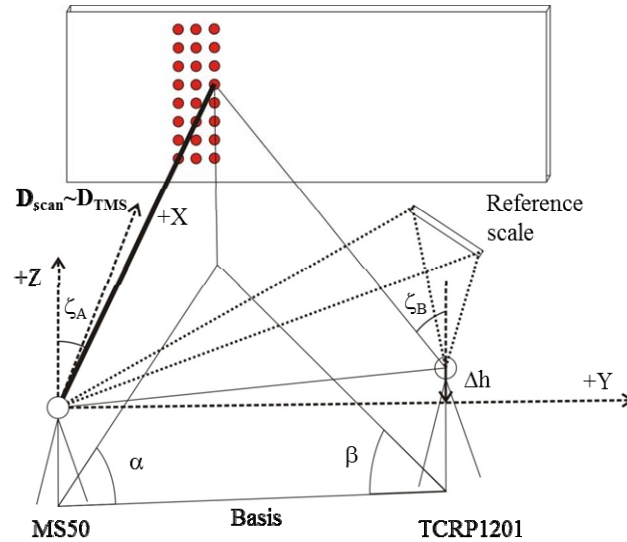
Fig. 1: Measurement setup
