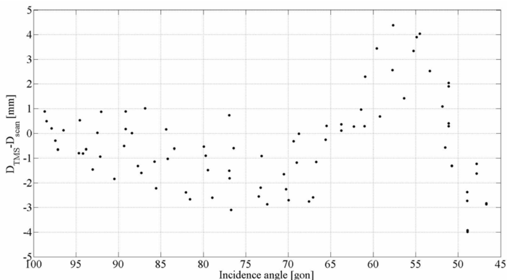
Fig. 3 Differences between D_{TMS} and D_{scan} as function of the angle of incidence
