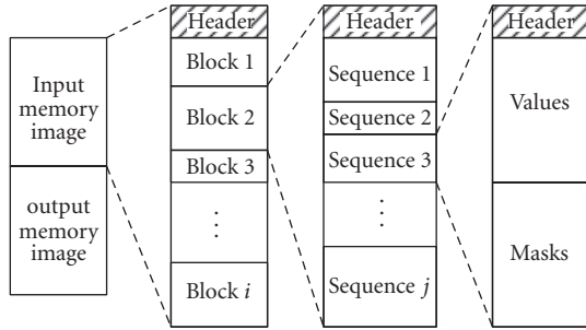
FIGURE 8: Structure of the memory image.
