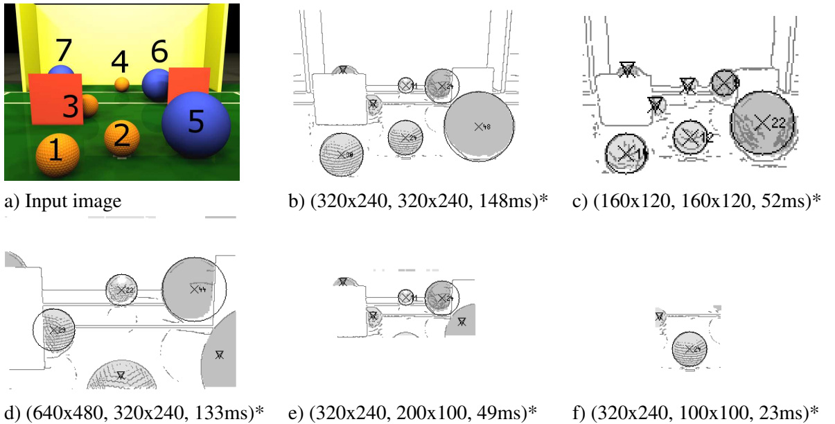
Figure 4: Image a) shows spheres of two different types on a virtual generated RobotCup-Soccer TeenSize playground. The images b) to e) represent the results with computation time by different resolutions and settings.
