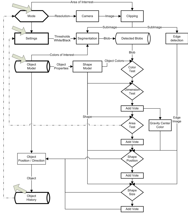
Figure 2: Data flow of the object detection. The large arrows mark the in- and output.
