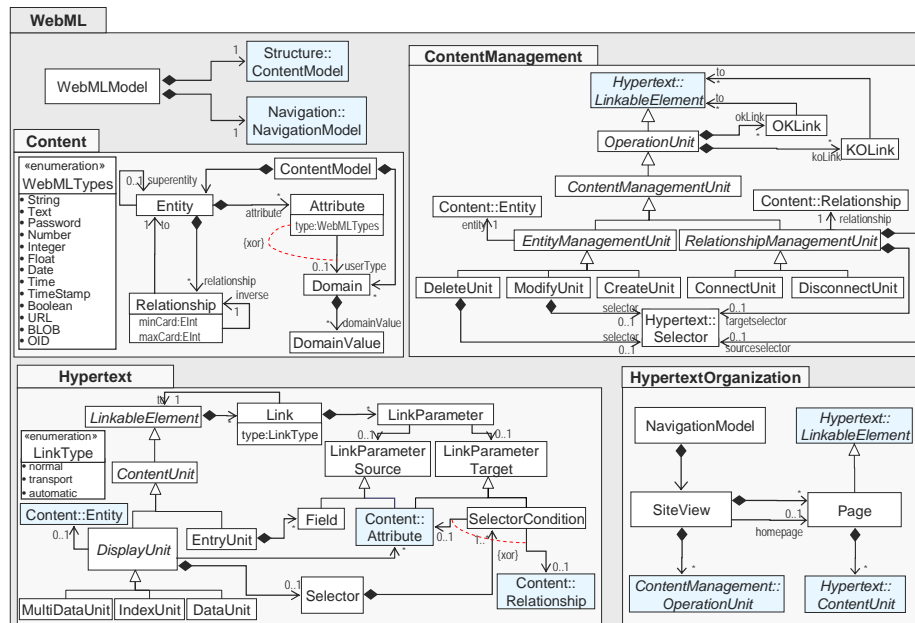
Figure 3: The WebML Metamodel
