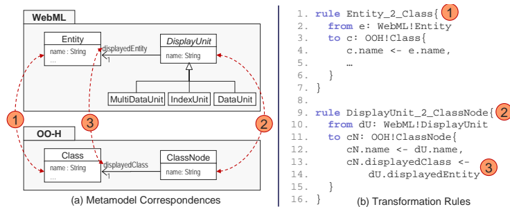
Figure 5: Metamodel Correspondences and Transformation Rules Excerpt
