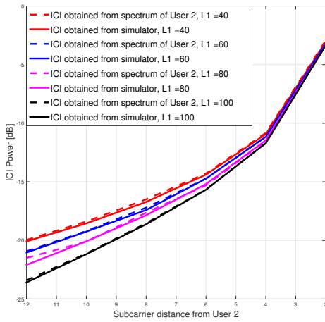
Figure 3: ICI at Receiver 1 obtained analytically and from simulation.
