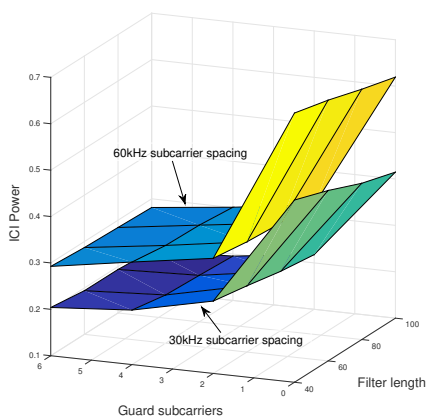
Figure 7: ICI at Receiver 2 for 30kHz and 60kHz subcarrier spacing.
