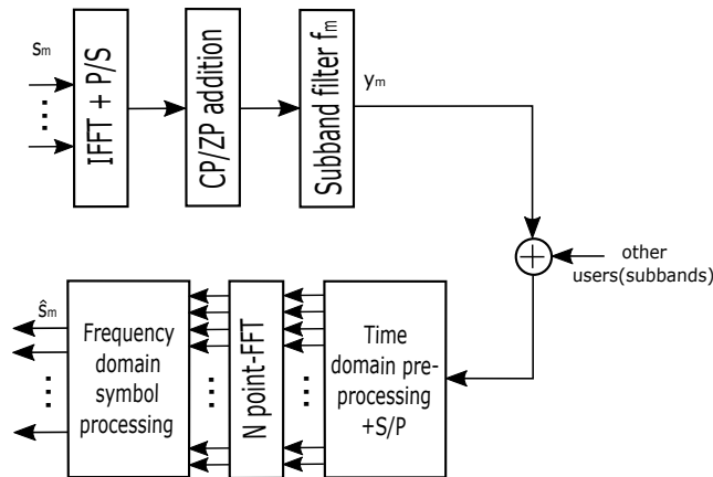
Figure 1: Basic UFMC transceiver
