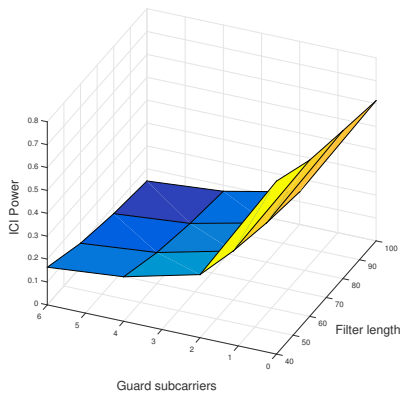
Figure 4: ICI at Receiver 1 in terms of guard subcarriers and filter length.
