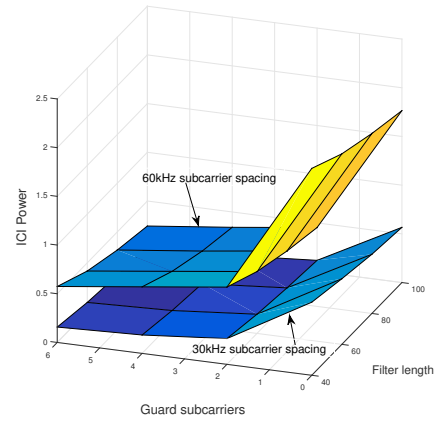
Figure 6: ICI at Receiver 1 for 30kHz and 60kHz subcarrier spacing.
