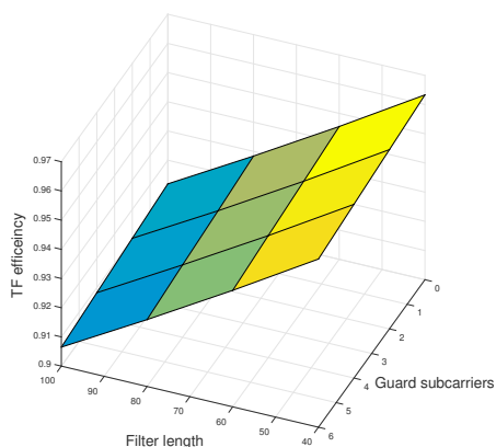
Figure 8: Time-frequency efficiency in terms of filter length and number of guard subcarriers.
