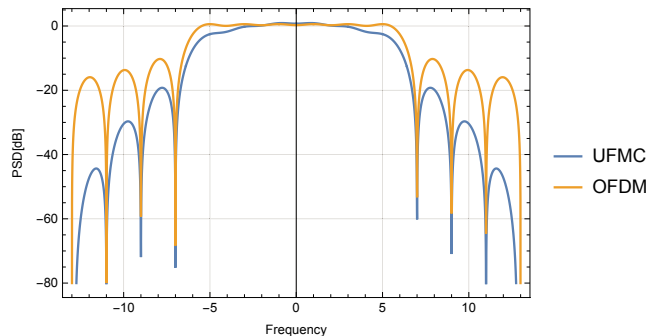
Figure 2: Spectrum of UFMC and OFDM signal of User 2.
