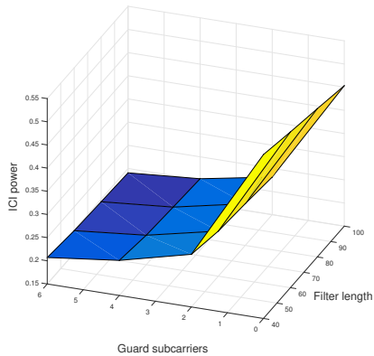
Figure 5: ICI at Receiver 2 in terms of guard subcarriers and filter length.
