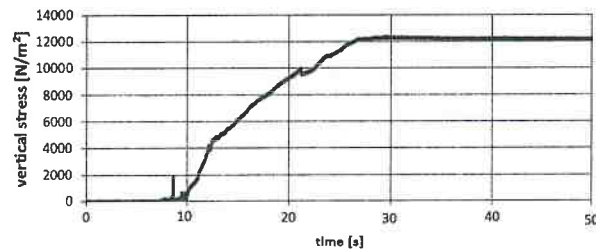
Figure 8. Vertical stress on the belt during filling, measured by use of the pressure sensor for direct measurement with a reduced cross-section of the hopper due to internals
