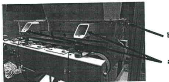
Figure 2. Test facility with load cells
