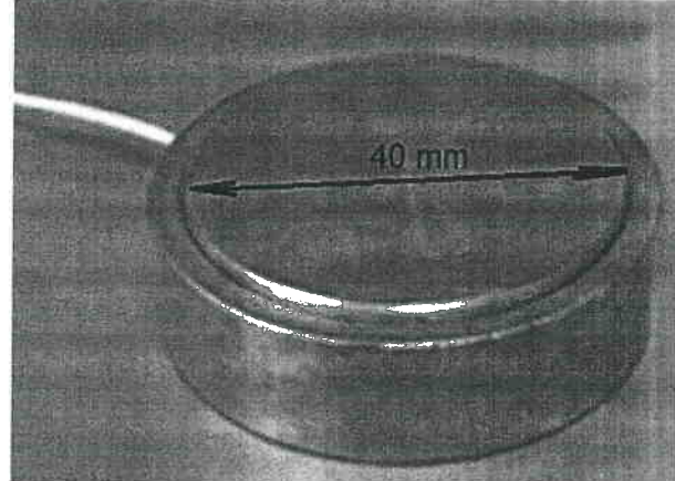
Figure 4. Pressure sensor for direct measurement of the vertical stress acting on the belt
