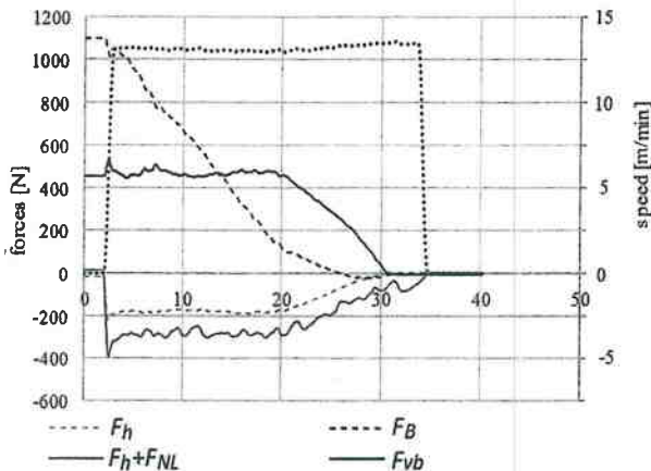
Figure 3. Horizontal and vertical forces acting on belt and hopper at emptying
