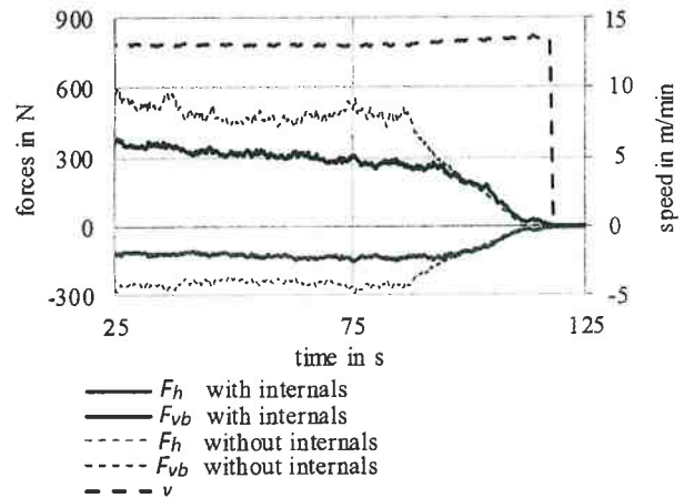
Figure 11. Emptying forces with and without internals at a outlet height of 30 mm
