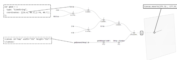
Fig. 2. The visualization of parts of the cartographic essence of a program as a result of the automatic analysis. Depicted here is a data flow graph of a single graphical attribute (the x coordinate of the endpoint of a line, derived from the longitude of a given point by an implementation of the Web Mercator projection). Each node in the data flow graph is either an arithmetic expressions or data con-version, and can be traced back to its location in the source code, facilitating closer inspection on demand.
