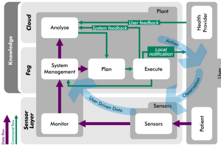
Fig. 4. HiCH: Our proposed IoT-based architecture.
