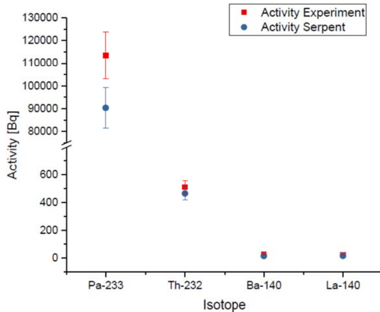
Figure 6 Calculated and experimental activity values of the Thorium-foil.
