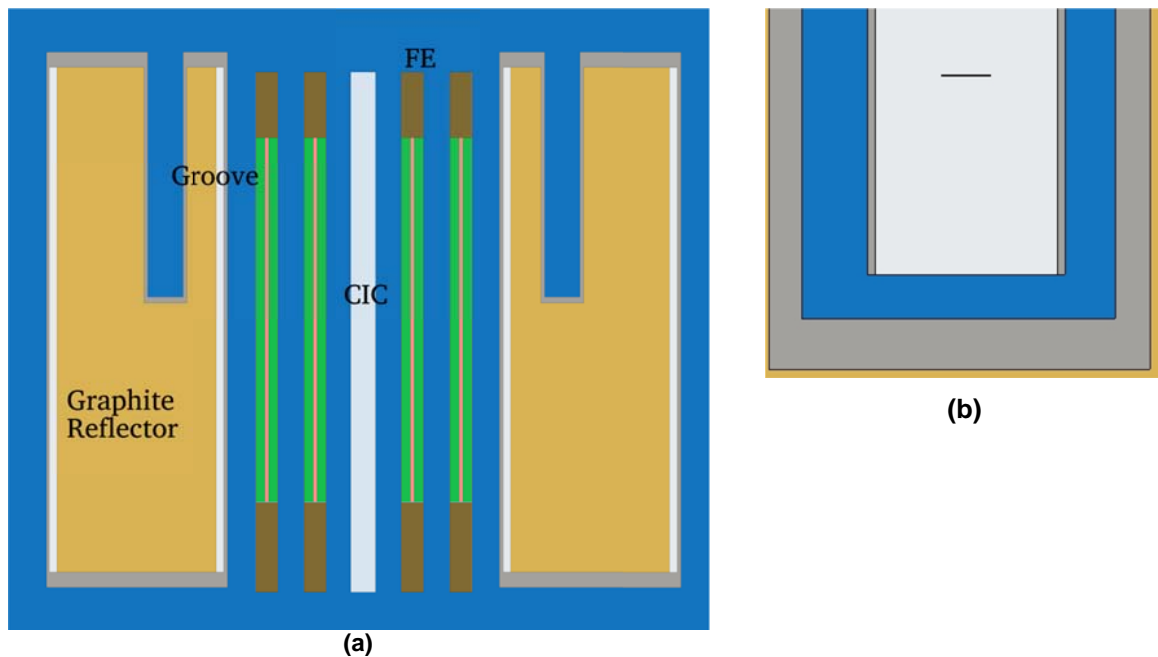
Figure 4: (a)The vertical section of the TRIGA core modeled with Serpent-2. (b) detail of irradiated foils in the LS1 irradiation position.
