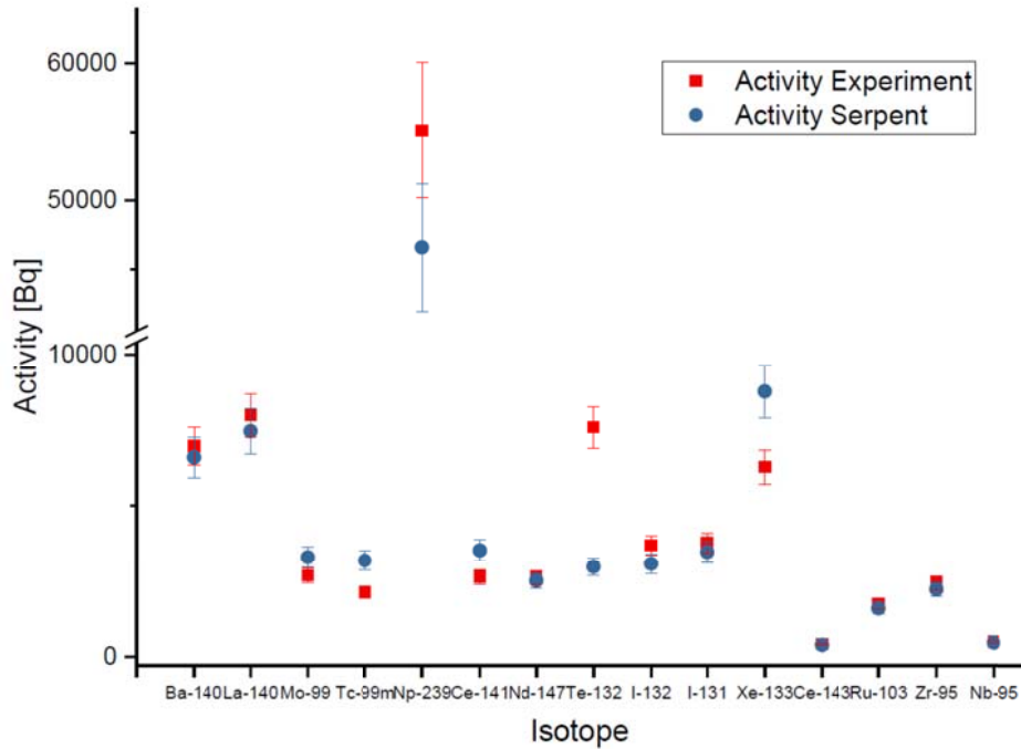
Figure 5: Calculated and experimental activity values of the Uranium-foil.
