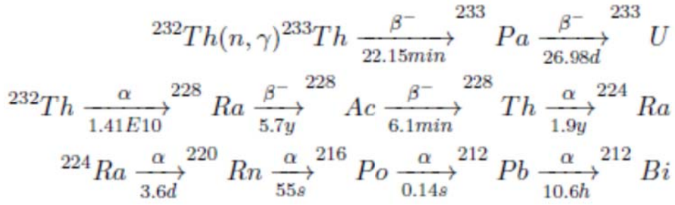
Figure 2: The capture reaction on Th-232 with its decay chain (up to U-233 production) and the natural Th-232 decay chain are shown.
