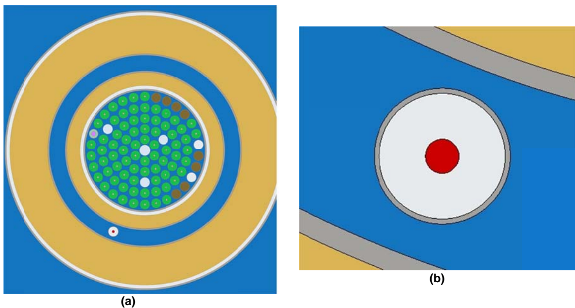
Figure 3: (a) The horizontal section of the TRIGA reactor model as obtained with Serpent-2 and (b) the detail of irradiation facility LS1 used for U and Th foils irradiation.
