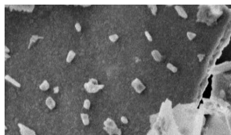
Figure 1. SEM: Fe Nanoparticle Exsolution from La 0.6 Ca 0.4 FeO 3
