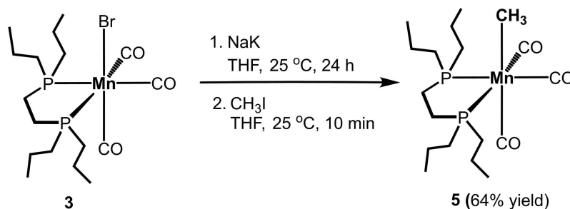
Scheme 3. Synthesis of \text{fac-}[\text{Mn}(\text{dpre})(\text{CO})_3(\text{CH}_3)] ( 5 ).
