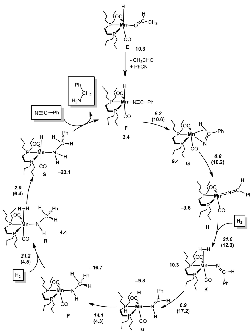
Figure 2. Simplified Catalytic Cycle for the Hydrogenation of Benzonitrile (Free energies in kcal/mol are referred to fac -[Mn(dpre)(CO) 3 (CH 3 )] ( 5 ), barriers in italic and transition state energies in parenthesis).
