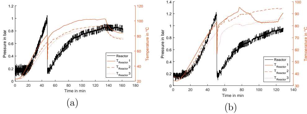
Figure 4.4: (a) Heating with 90-100 % of maximum heating power. The system was evacuated again when the reactor pressure exceeded 1 bar. The temperature in the reactor does not exceed 100 °C. (b) Heating conditions like in (a), but with additional insulation.
