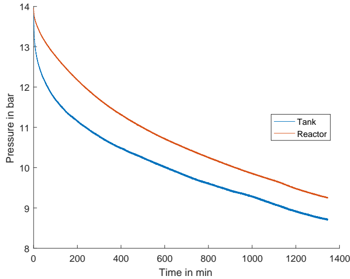
Figure 4.2: Pressure loss during a 24 h compressive strength test
