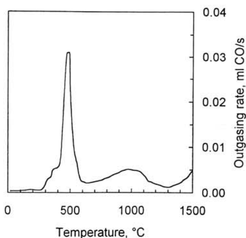
Fig. 3. CO formation of a Fe(0.4%O)-TiC composite.
