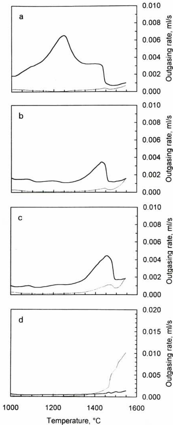
Fig. 6. Outgassing behaviour of Fe-TiC x N 1-x composites (a: Fe-TiC 0.7 N 0.3 ; b: Fe-TiC 0.5 N 0.5 ; c: Fe-TiC 0.3 N 0.7 ; d: Fe-TiN), thick line represents CO and the thin line represents N 2 formation.
