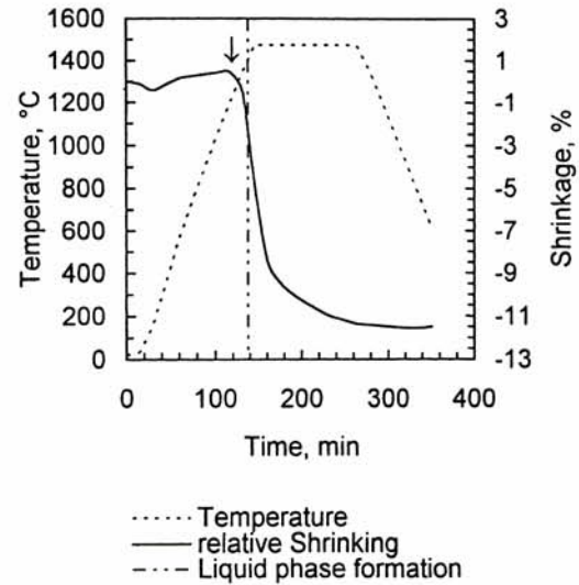
Fig. 7. Dilatometric measurement of a Fe-TiC 0.7 N 0.3 composite, heated at a rate of 10 K/min up to 1475°C and held for 2 h. The shrinking starts more than 200°C below the formation of the liquid phase.
