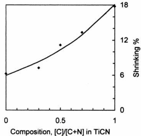
Fig. 8. Shrinking during sintering Fe-TiC x N 1-x composites up to 1550°C at a rate of 25 K/min as a function of the [C]/[C + N] ratio in the hard phase.
