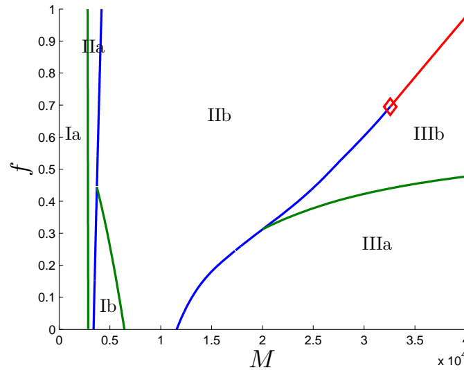
Fig. 5: This figure shows the different regions in the M - f space. The green lines denote continuous transitions from region I to II ( R_0 = 4 ). The blue curve is a Skiba curve, where the transition from region II to III is discontinuous, and exactly on the Skiba curve two optimal solutions exist. The Skiba curve switches to a continuous transition curve (red line) at the red diamond. In Regime IIIb the lockdown is imposed then relaxed and then tightened again, whereas in Regime IIIa the lockdown is steadily increased and then steadily relaxed.
