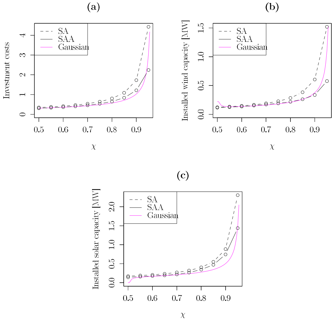
Figure 2.2: Fig. (a) shows the expected invested capital in units of 10^6\text{€} for different levels of reliability. Fig. (b) and (c) show the installed capacities for wind and solar technology.
