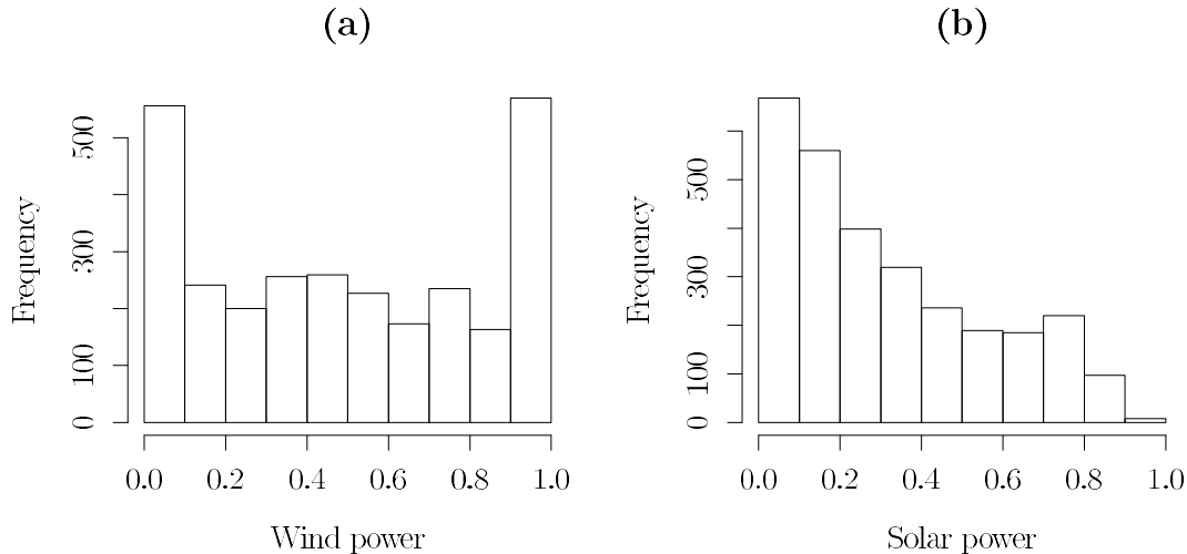
Figure 2.1: Histograms of the hourly values of the power per installed capacity in the daytime for (a) wind and (b) solar power for one sampled year. The values are given in MW for one MW of installed capacity.
