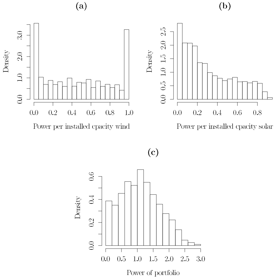
Figure 3.1: Fig. (a) shows a histogram of the wind power per installed capacity. Fig. (b) shows a histogram of the solar power per installed capacity, both for typical locations in Central Europe. Fig. (c) illustrates the distribution of the power available for an energy portfolio of 1 MW installed wind capacity and 2 MW installed solar capacity.
