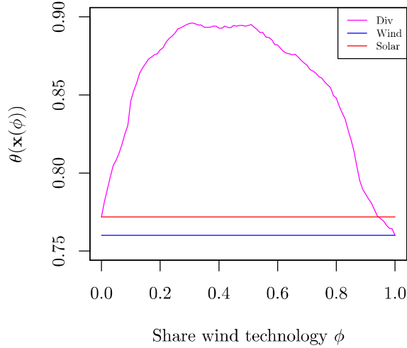
Figure 3.9: This figure demonstrates the quasi-concavity of the distribution function in an example.
