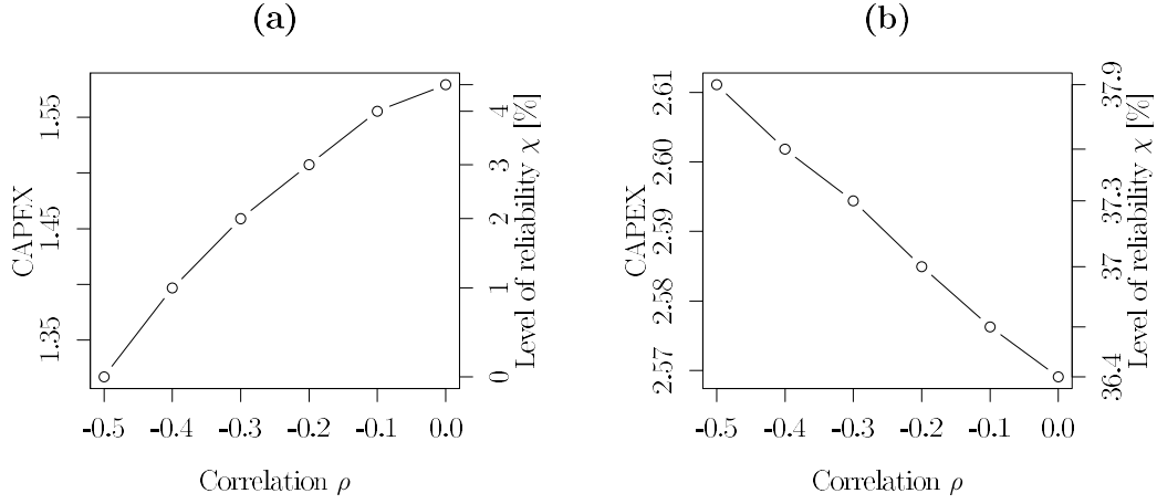
Figure 3.8: This Figure shows the energy manager’s optimal investment decision in RES, when the energy price at the balancing market is correlated with the cumulated RES power output. Both plots represent the situation of the high price scenario of the investment goods. Fig. (a) shows the optimal level of investment, when the mean energy price is \mu' = 40\text{€}/MWh and spot price risk is \sigma' = 40\text{€}/MWh . Fig. (b) shows the optimal level of investment for \mu' = 100\text{€}/MWh and a spot price risk of \sigma' = 40\text{€}/MWh .
