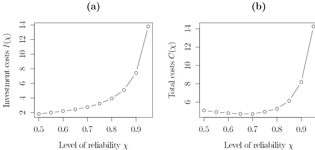
Figure 3.4: Fig. (a) shows the energy manager’s optimal investment frontier for different values of the reliability parameter. The costs of investment is given in units of 10^6\text{€} . Fig. (b) shows a simulation of the total costs when the expected costs for a shortfall of the power supply are integrated and a shortfall in the power supply is penalized with 200\text{€}/MWh .
