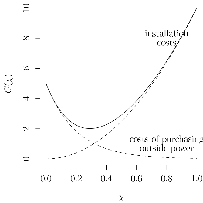
Figure 3.2: Illustration of the total costs associated with the energy park as a function of the confidence parameter \chi of the supply demand constraint.
