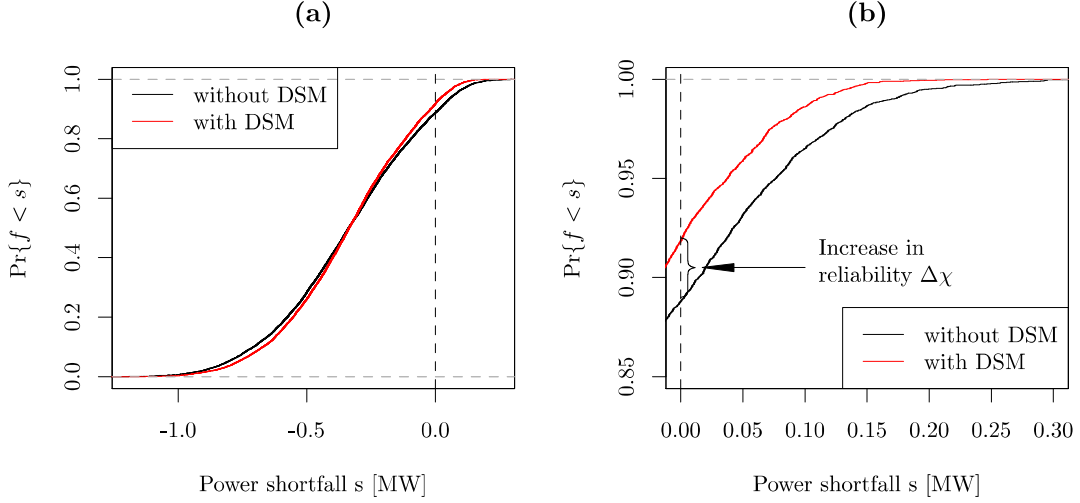
Figure 2.6: Fig. (a) shows the empirical cdf for the ex-ante optimal investment strategy associated without DSM in two cases: (i) without DSM (black line) and (ii) with ex-post DSM adjustment, Fig. (b) shows a section of plot (a) to illustrate the increase in reliability, when DSM is included. The plots are given for \mu_d = 0.1MW, \sigma_d = 0.1MW, \rho = 0.5 and \chi = 0.9 .
