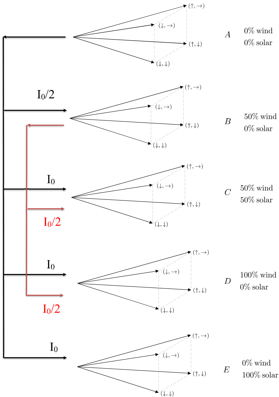
Figure 4.4: This figure illustrates all possible energy portfolios of wind and solar technology considered. The arrows illustrate the flexibility options (black: flexibility options when no investment has occurred, red: flexibility options when a partial investment in wind technology has occurred).
