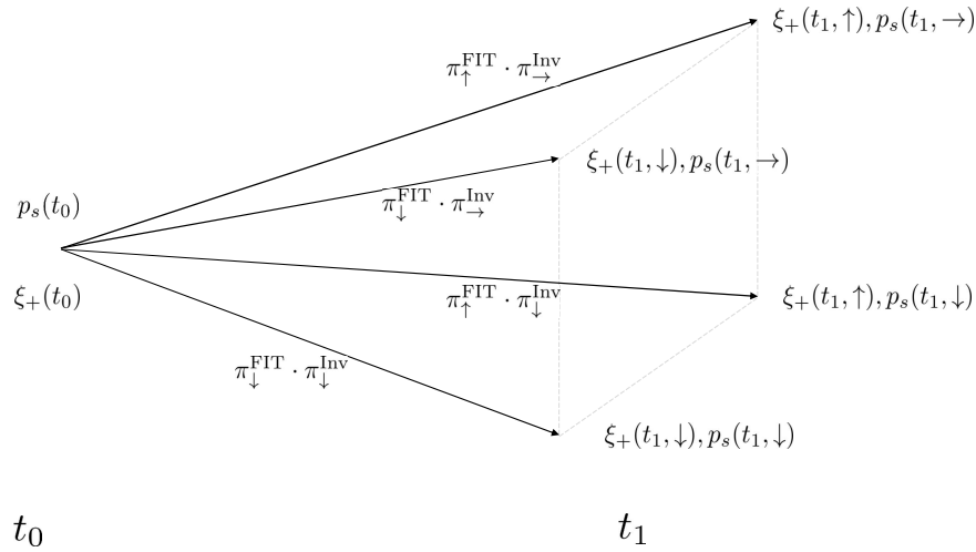
Figure 4.3: This figure represents the joint grid of the states of nature in the one-step problem with the 4 possible states arising in the future.
