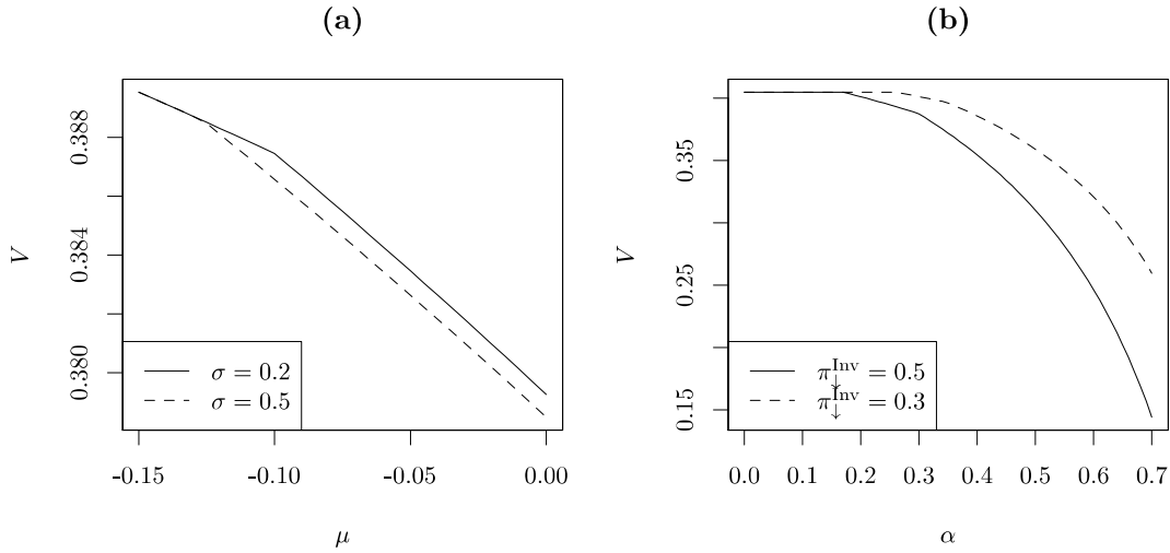
Figure 4.5: Figure (a) shows the value of the option to invest in RES as a function of the drift rate \mu for two levels of \sigma ( \alpha = 0.3 , \pi_{\downarrow}^{\text{Inv}} = 0.5 ). Figure (b) shows the value of the option as a function of the level of the innovation in solar technology for two levels of the probability to obtain an innovation in the next period ( \mu = -0.1 , \sigma = 0.2 ).
