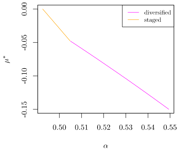
Figure 4.8: This figure shows the relationship between the level of innovation in solar technology and the endogenized drift rate \mu^* s.t. the energy manager is indifferent in investing now or to defer the investment decision. The impact of the probability to obtain an innovation in solar technology is also demonstrated. In this numerical example \sigma = 0.2 , \pi_{\downarrow}^{\text{Inv}} = 0.1 and \xi_- = 100\text{€}/MWh are chosen.
